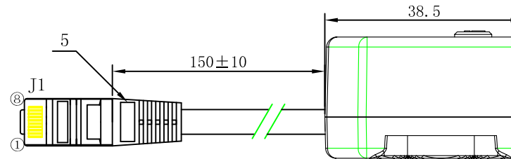
Network wire stripping and heat shrinkable pipe installation schematic diagram.
